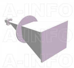
LB-62-25-C2-SFSPO Standard Gain Horn Antenna 12.4-18GHz 25dB Gain SMA Female
