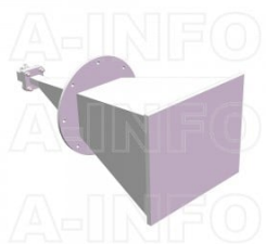
LB-62-25-C2-3.5FSPO Standard Gain Horn Antenna 12.4-18GHz 25dB Gain 3.5mm Female
